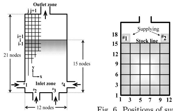
Fig. 6. Positions of supplying materials
