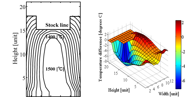
(c) Estimated temperature distribution (d) Temperature difference distribution
