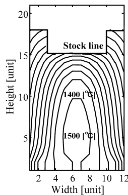
Fig. 12. Desired temperature distribution
