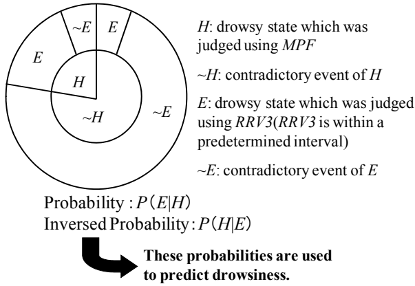
Fig.2 Explanation for calculating inversed probability P(H|E) on the basis of Bayesian theorem.
