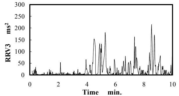
Fig.4: An example of time series of RRV.
