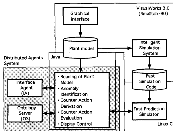
Fig. 1 Configuration of semantic representation interface and relation with other intelligent agents.
