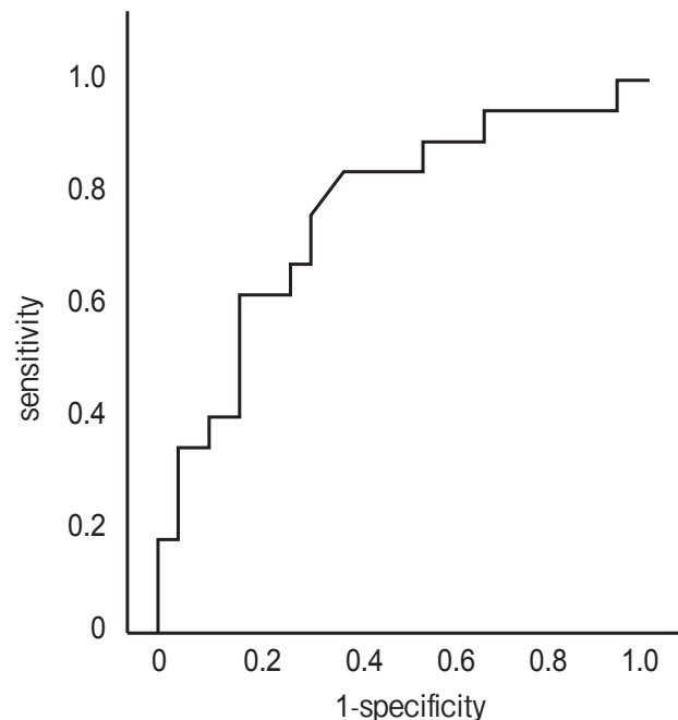
Fig. 2 The ROC curve revealed that the preoperative cut-off time of 15.3 sec for the Timed "Up and Go" (TUG) test was sensitive (83.3%) and specific (61.1%) for a deep venous thrombosis complication after total hip arthroplasty.
