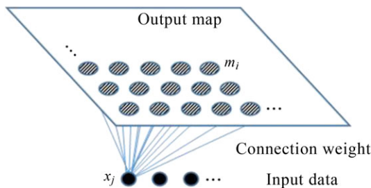
Fig. 1. Structure of a self-organizing map (SOM). m_i is i th unit in output map. x_j is j th input data.
